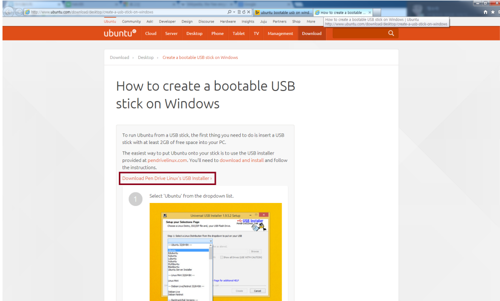
사진 33: http://www.ubuntu.com/download/desktop/create-a-usb-stick-on-windows
